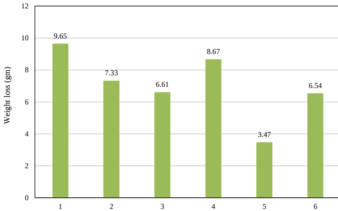
Fig. 4. Results of weight loss due to abrasion (gm).
