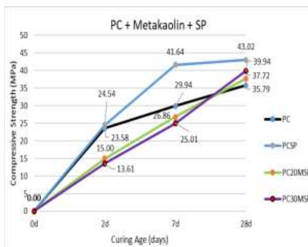
Fig. 3b Compressive Strength of PC and Metakaolin at 2, 7, 28 days
