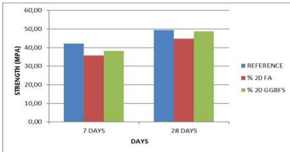
Fig. 2. Compressive Strength
