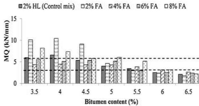
Fig. 1. Marshall Quotient's comparison of different fly ash content and 2% hydrated lime containing mix. [6]
