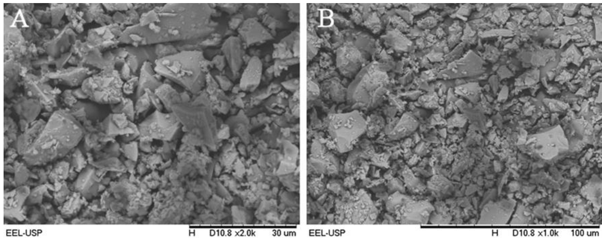
Figure 1. SEM micrograph of Portland cement: (a) 2.0 kx; (b) 1.0 kx.
