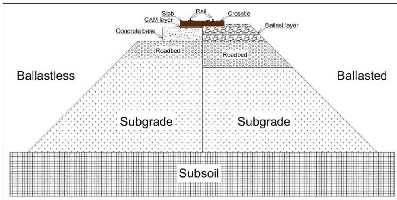
Figure 5. Ballastless and Ballasted High Speed Railway Line.
