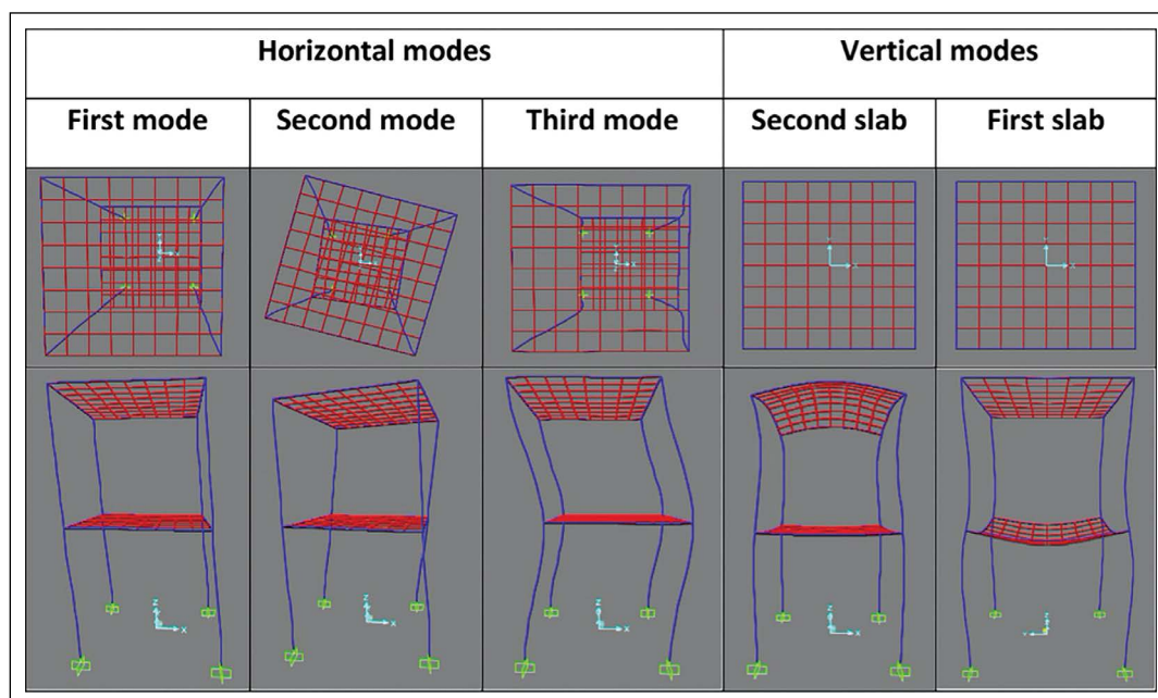
Figure 29. Modal configurations [44].
