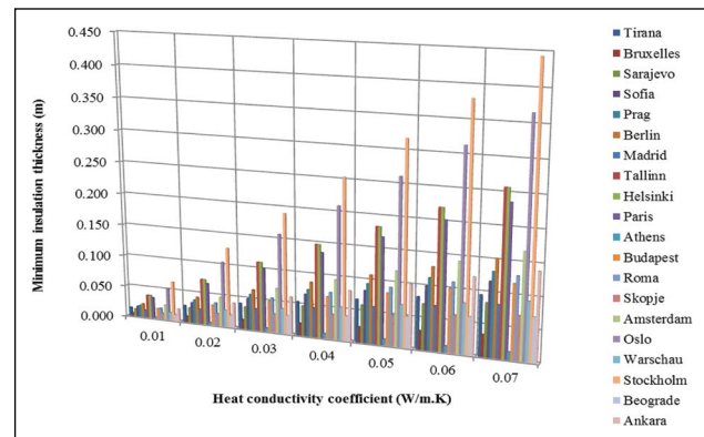
Figure 3. Minimum insulation thicknesses for floor depending on different heat conductivity coefficients.
