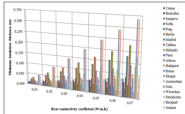
Figure 1. Minimum insulation thicknesses for external wall depending on different heat conductivity coefficients.
