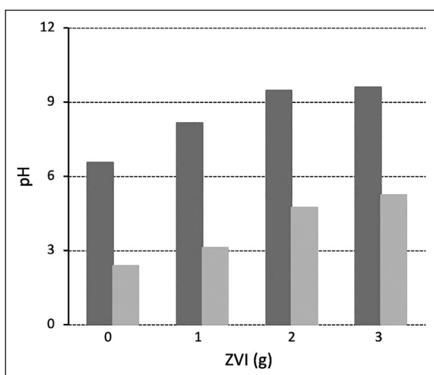
Figure 5. Final pH values of solutions in batch Bechamp reduction after 7 hours, as a function of ZVI: without acid (dark grey); with 1 % \text{H}_3\text{PO}_4 (light grey).
