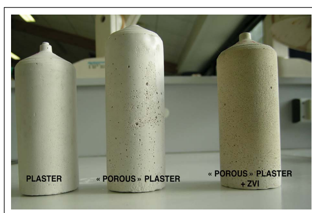
Figure 6. Plaster column composition: plaster (50.0 g, 41.0%); water (57.4%); \text{CaCO}_3 (0.2%); \text{H}_3\text{PO}_4 (1.4%); ZVI (2.3%).
