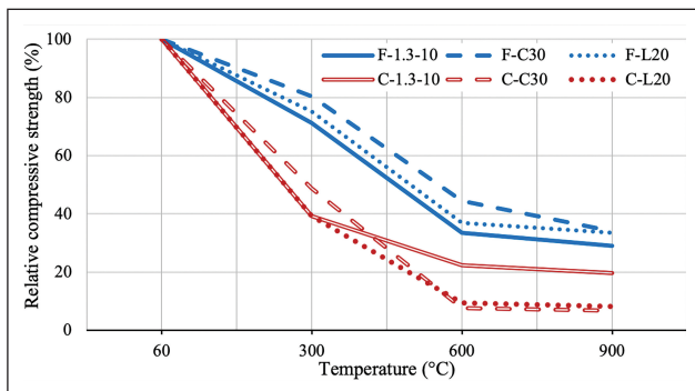
Figure 9. Relative compressive strength of geopolymer mortars exposed to high temperatures.
