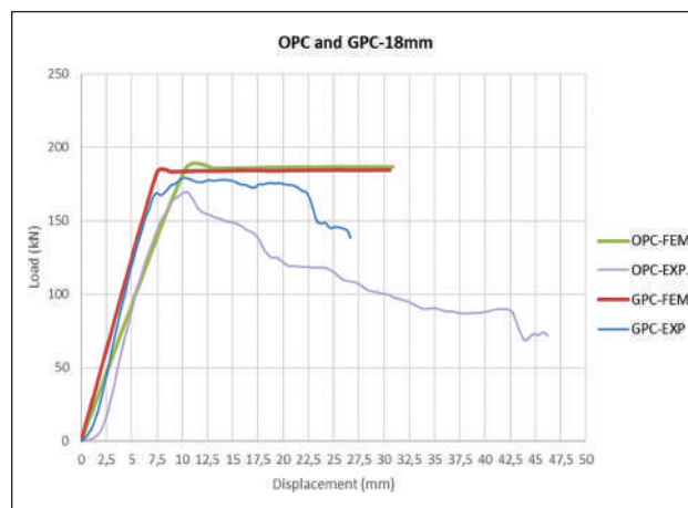
Figure 8. Stress-strain curves (OPC and GPC 18 mm).
