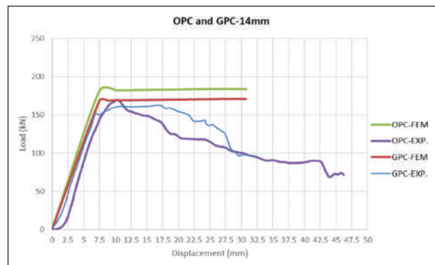
Figure 6. Stress strain curves (OPC and GPC 14 mm).
