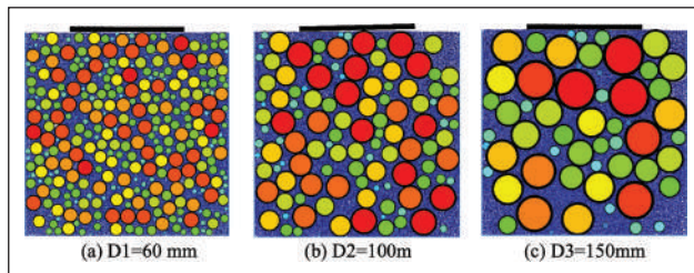
Figure 10. Models with different maximum particle size.
