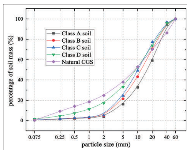
Figure 2. Gradation curves of test soil samples.
