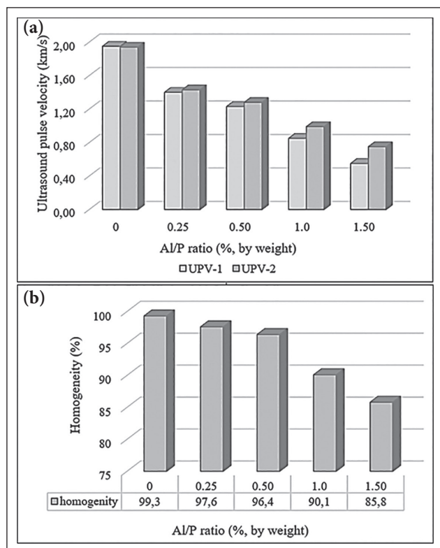
Figure 11. (a) Ultrasound pulse velocity obtained from two different regions in a sample; (b) calculated homogeneity percentage.
