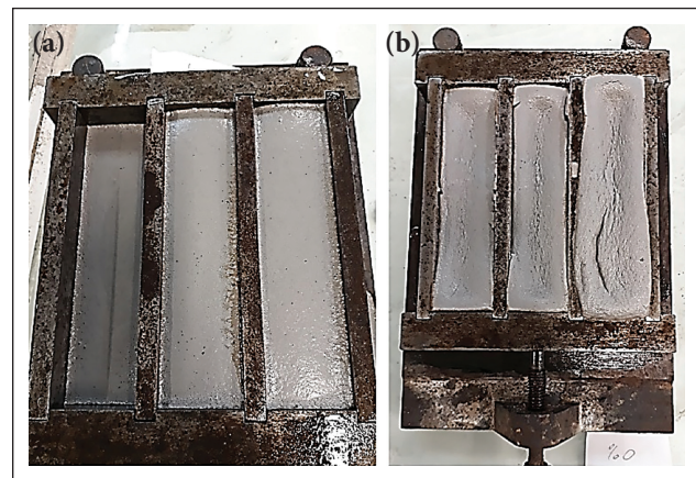
Figure 3. (a) The specimens 10 minutes after placing the molds; (b) The existence of collapse 30 minutes after placing the molds.
