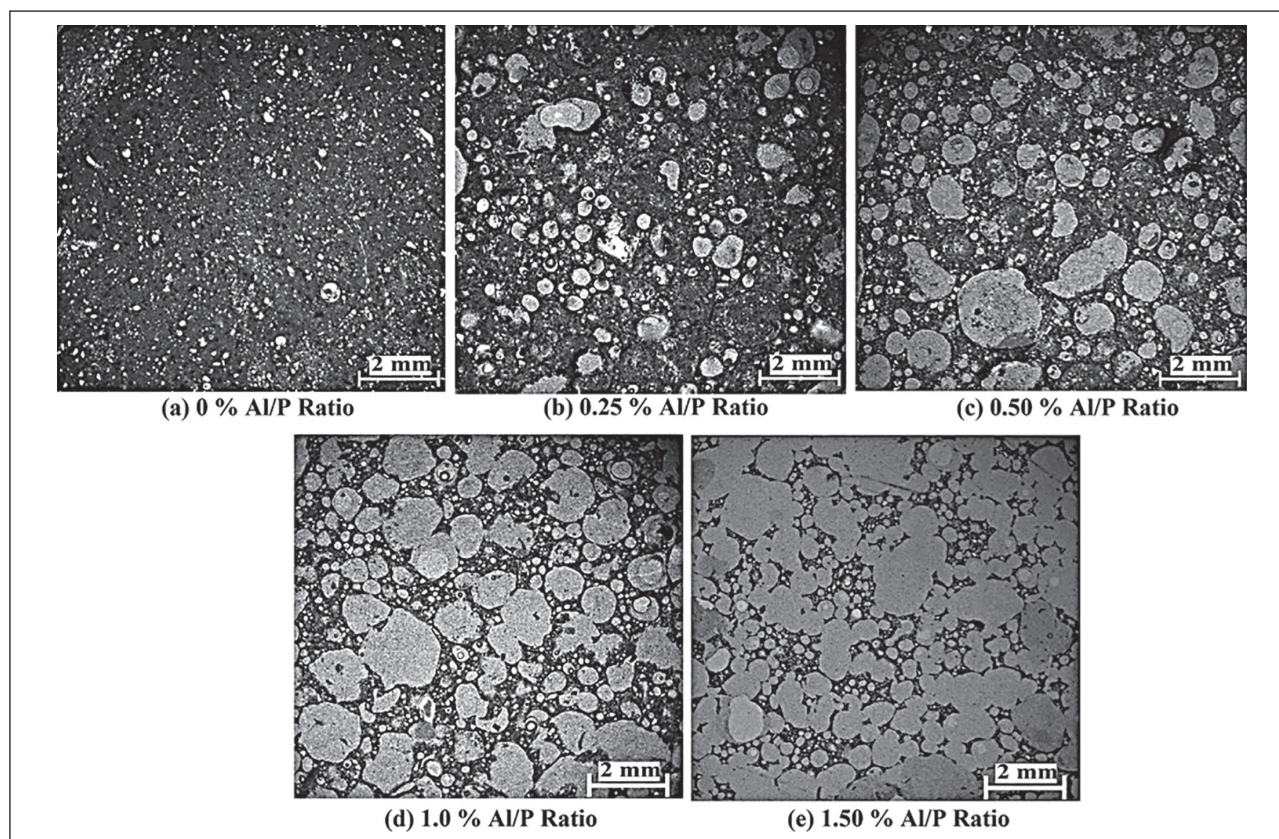
Figure 9. Microscopic images of ED-based geopolymer foams having various Al/P ratios.
