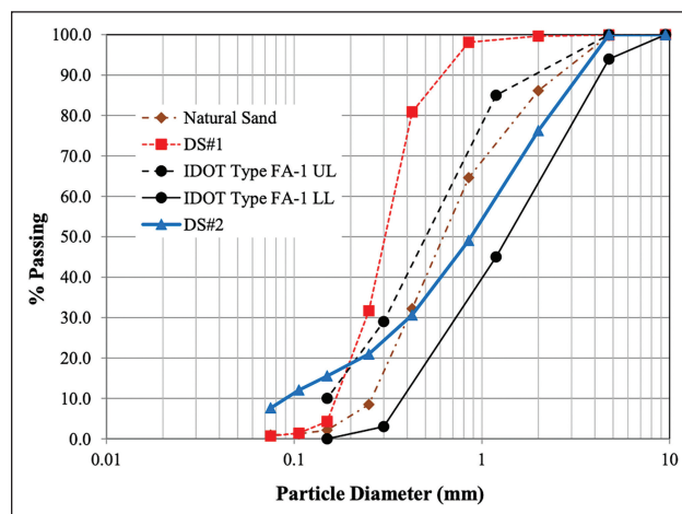
Figure 2. Sieve analysis results.
