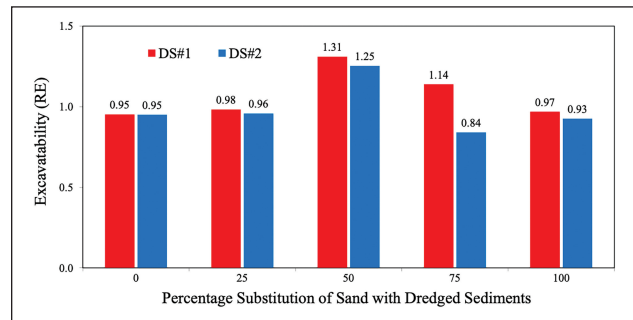
Figure 8. Variation of excavatability with percentage substitution of sand with dredged material.
