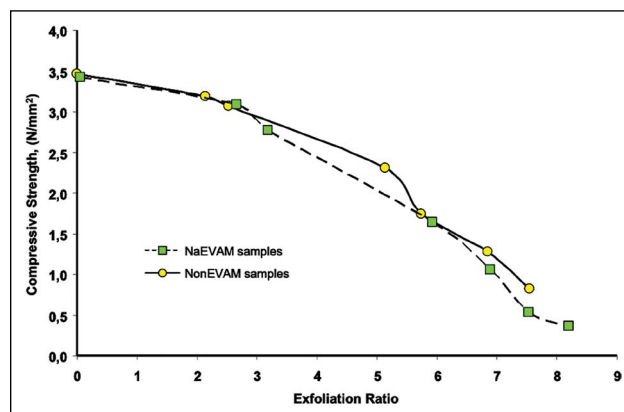
Figure 6. Effects of exfoliation ratio to the compressive strength of EVAM samples at the equilibrium stage.
