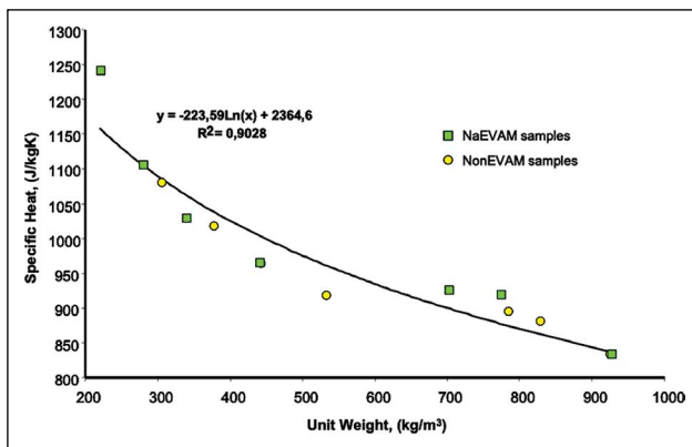
Figure 8. Density versus Cp value of tested samples.
