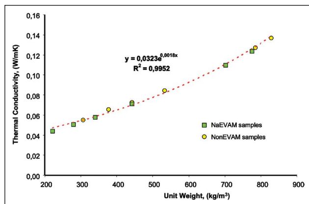
Figure 7. Density and thermal conductivity relationship.
