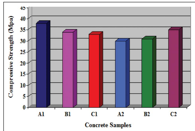
Figure 17. Compressive strength of concrete samples after immersion in tap water [66].
