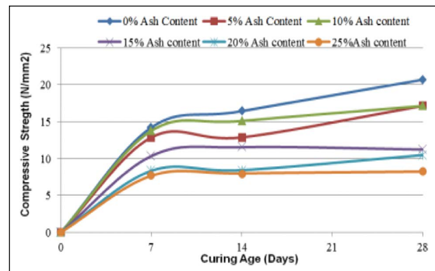
Figure 9b. Cement-PPA concrete compressive strength [51].
