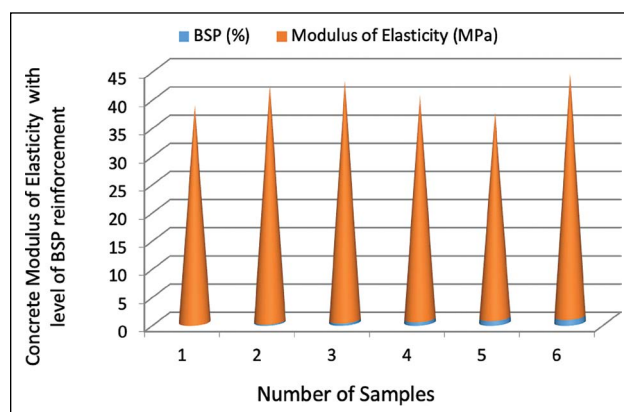
Figure 13. Concrete modulus of elasticity with the level of BSP reinforcement [62].
