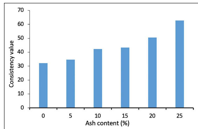
Figure 6. Consistency of cement paste at different percentages of PPA included [51].
