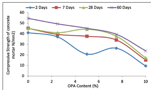
Figure 18. Effect of OPA on mortar compressive strength [64].
