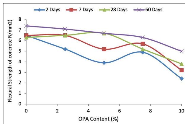
Figure 20. Flexural strength of concrete blended OPA [64].
