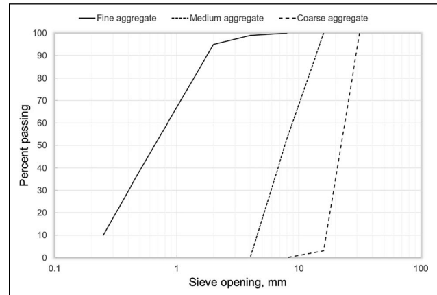
Figure 1. Sieve analysis results of natural aggregates.
