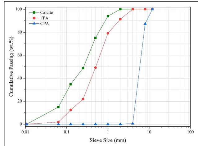
Figure 2. Sieve analysis of calcite, FPA, and CPA.
