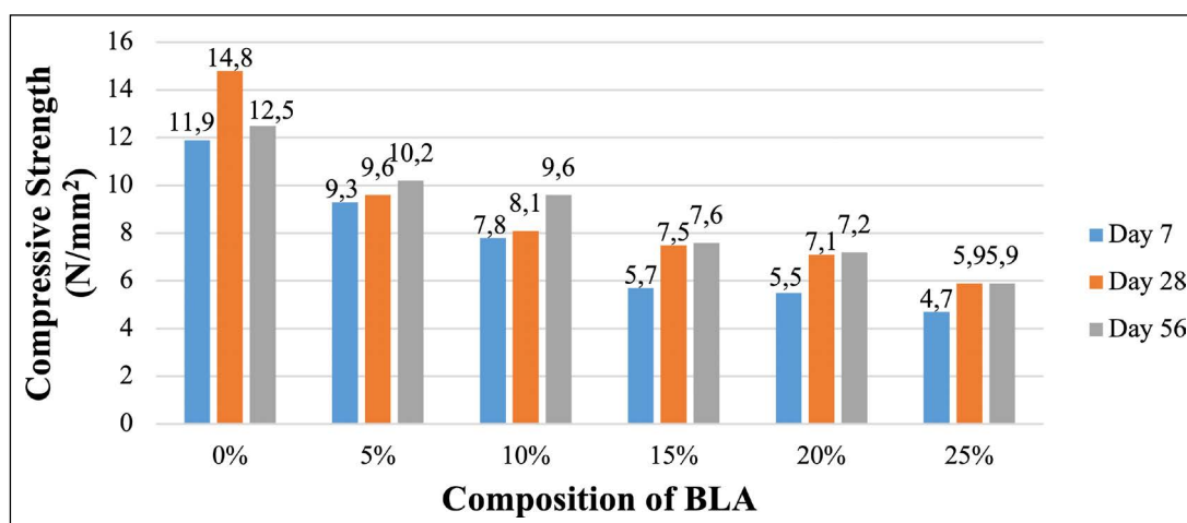
Figure 5. A graph showing the comparison of the average compressive strengths of concrete at 7, 28 and 56 days against the composition of BLA in cement.
