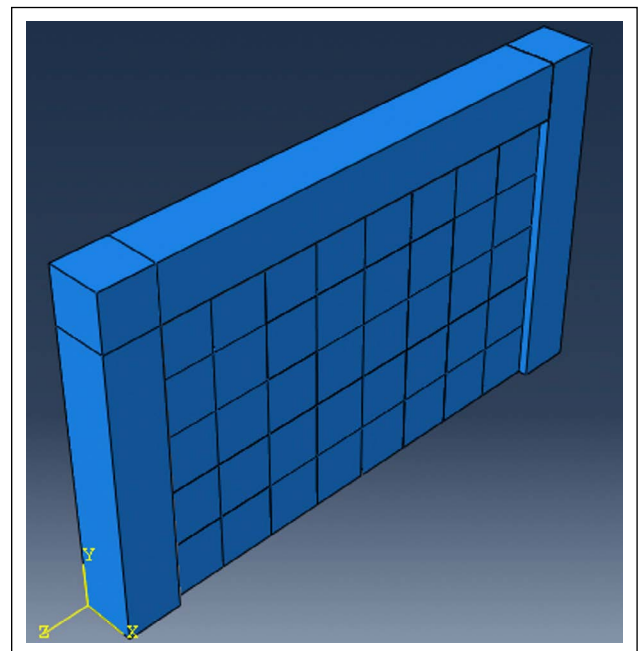
Figure 2. Demonstration of Abaqus modeling of RC frame with infill wall and attached panels.
