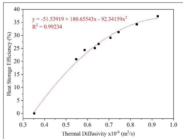
Figure 12. Relation between heat storage efficiency and thermal diffusivity of SLCs.
