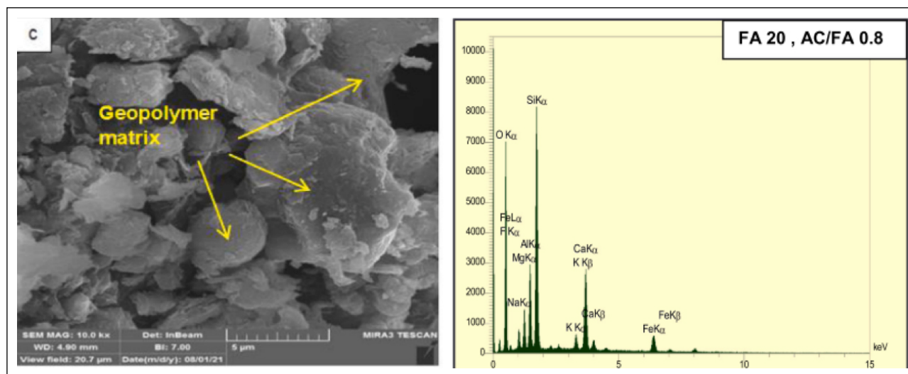
Figure 6. SEM-EDS analysis for geopolymer-treated clay soil [126].
