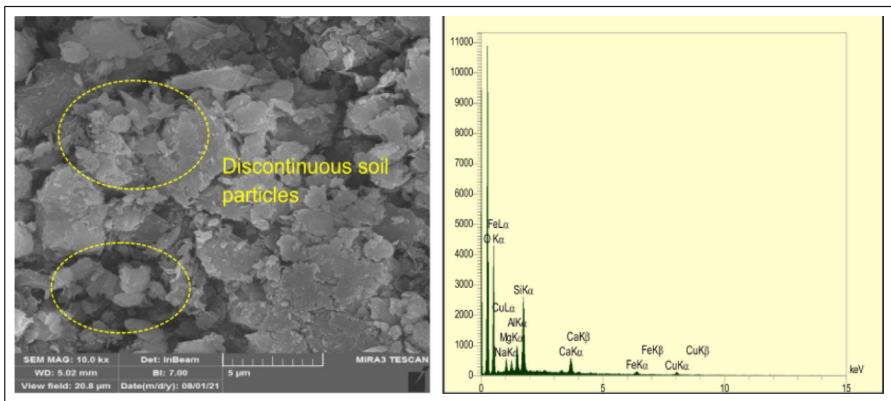
Figure 4. SEM-EDS analysis of untreated clay soil [126].
