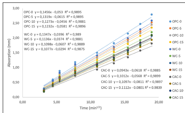
Figure 15. Sorptivity coefficient results after 90 freeze-thaw cycles.
