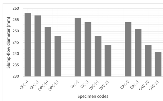
Figure 2. Slump-flow diameters of mixtures.
