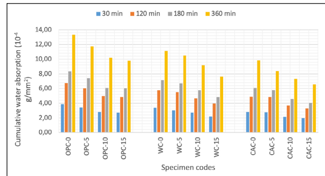
Figure 5. Cumulative capillary water absorption results of mixtures.
