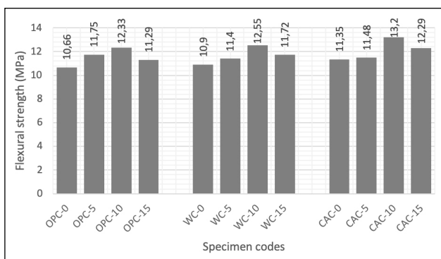
Figure 4. Flexural strength results of mixtures.
