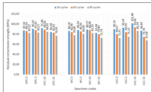
Figure 8. Residual compressive strengths after freeze-thaw.
