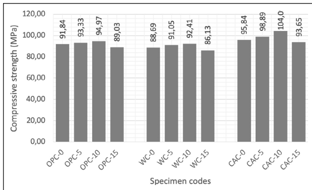
Figure 3. Compressive strength results of mixtures.
