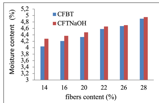
Figure 5. Moisture content as a function of fibers content.
