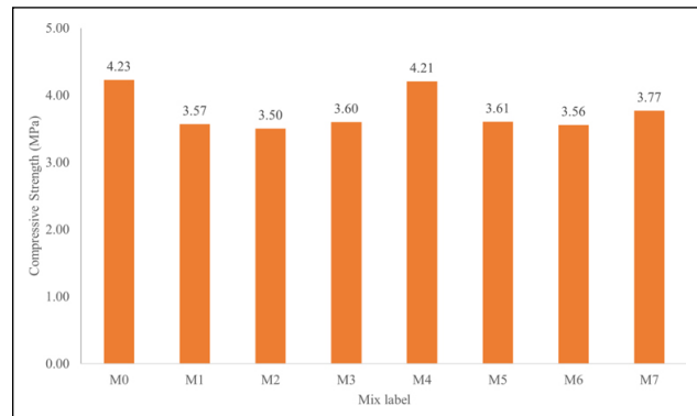
Figure 5. Compressive strength.
