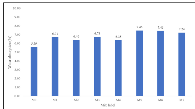
Figure 6. Water absorption.
