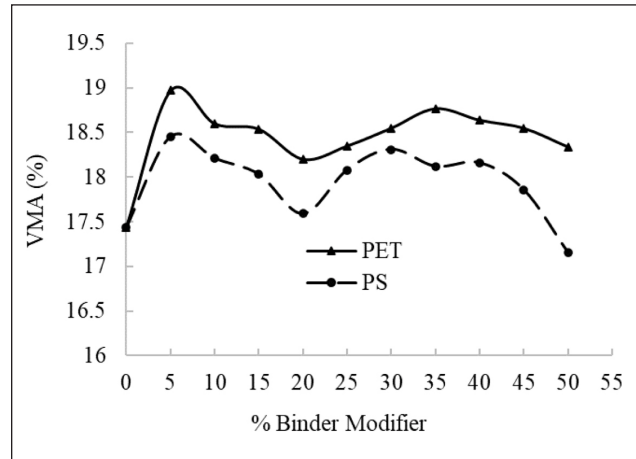
Figure 13. Influence of modifiers on voids in mineral aggregate.
