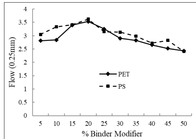
Figure 10. Influence of modifiers on Marshal flow values.
