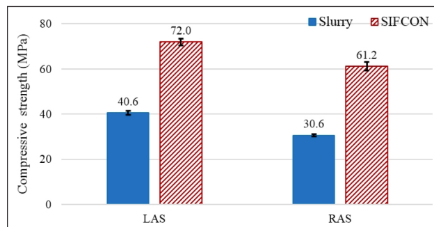
Figure 7. Compressive strengths of slurries and SIFCONs.
