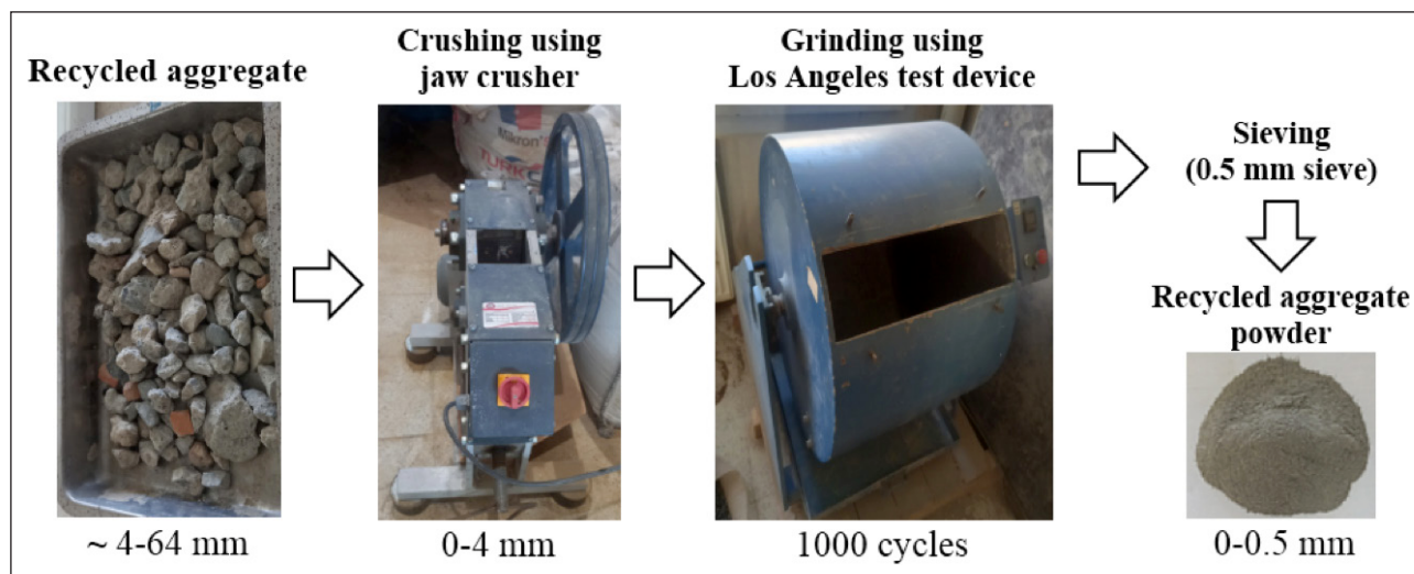
Figure 1. Preparation of RA powder.
