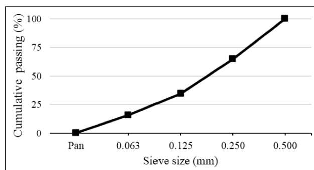
Figure 3. Gradation of aggregates.
