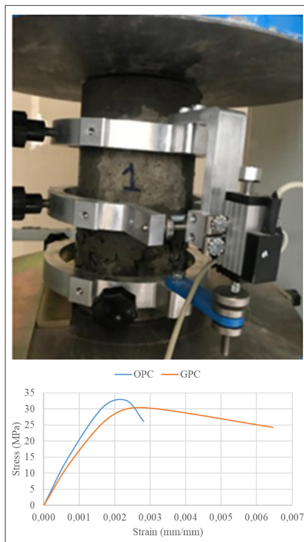
Figure 5. Stress-strain curves.
