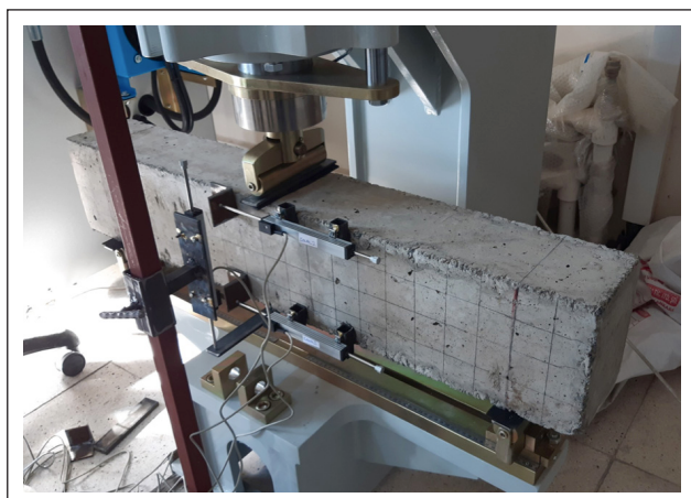
Figure 3. Experiment setup and measuring instruments.
