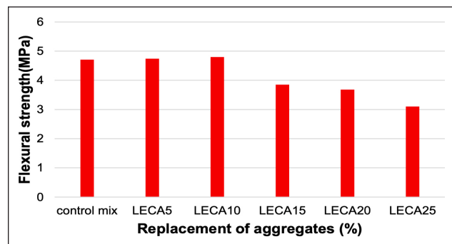
Figure 5. Flexural strength of concrete of different replacements.
