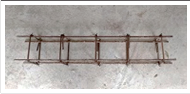
Figure 3. Reinforcement bars.
