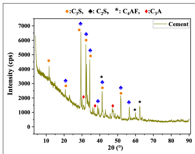
Figure 2. XRD pattern of the cement.
