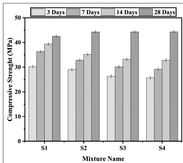
Figure 4. Compressive strength bar graphs of different mortar series for 3, 7, 14, and 28 days.
