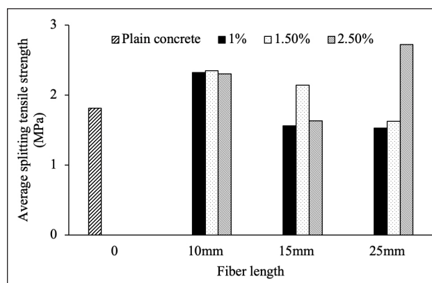
Figure 3. Relationship exhibiting the influence of the fiber volume and length on the average splitting tensile strength of KFRC specimens.
