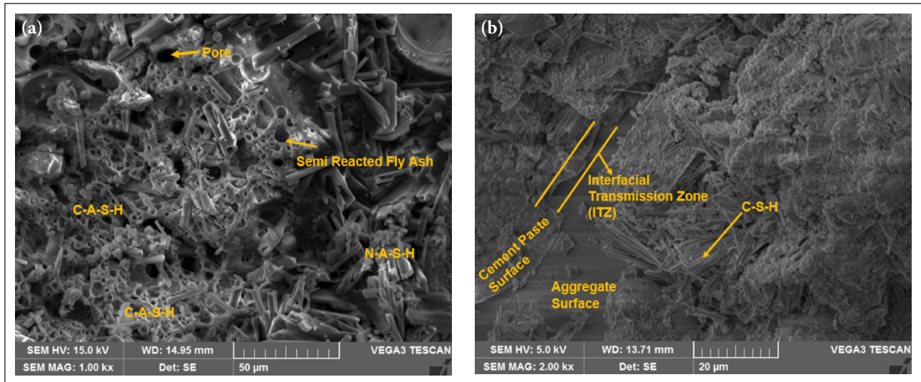
Figure 8. (a) S.E.M. of 80% F.A. + 20% oven-dried GGBFS geopolymer aggregates. (b) SEM of M3 concrete mix.
