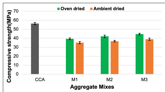
Figure 9. Compressive strength results.
