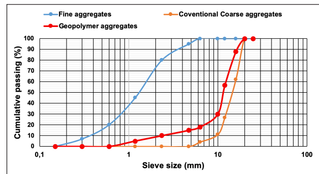
Figure 2. Grading curves of aggregates.
