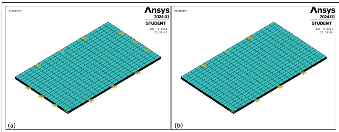
Figure 5. Meshed FGM rectangular plates with (a) CCCC and (b) CCFF boundary conditions.
