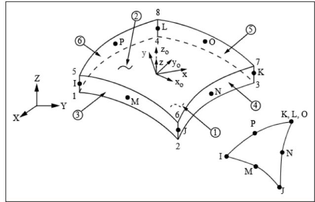
Figure 3. SHELL281 geometry [58].
