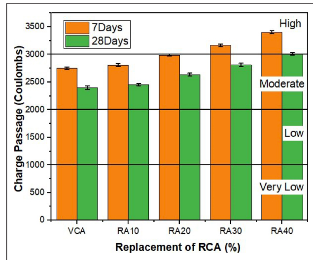
Figure 9. Chloride ions passage of RCA-based Geopolymer concrete.
