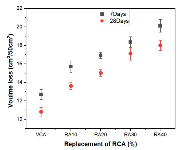
Figure 8. Abrasion resistance of RCA-based Geopolymer concrete.
