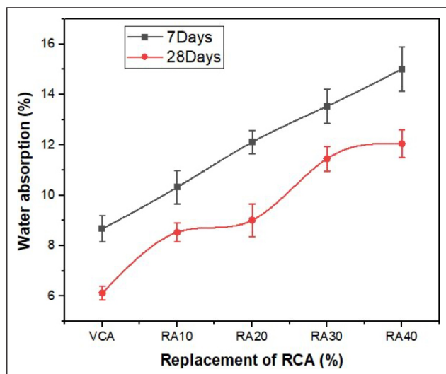
Figure 7. Water absorption of RCA-based Geopolymer concrete.
