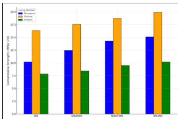
Figure 4. Compressive strength of GMs under different curing methods.
