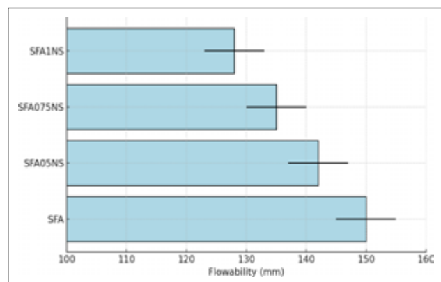
Figure 2. Flowability of GMs under different curing methods.
