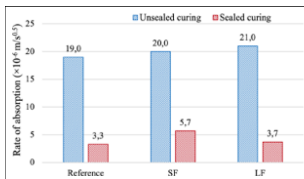
Figure 11. Initial rate of water absorption values.
