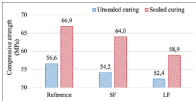
Figure 4. Compressive strength test results.
