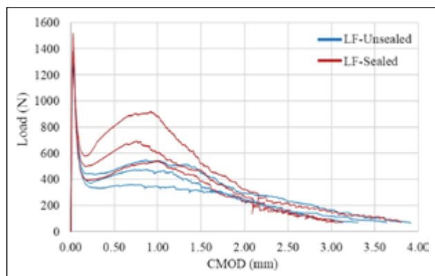
Figure 7. Load-CMOD curves of long fiber-reinforced mortars.
