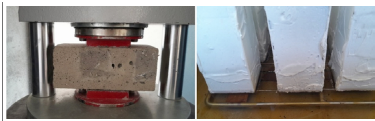
Figure 3. Compressive strength and sorptivity test photographs.
