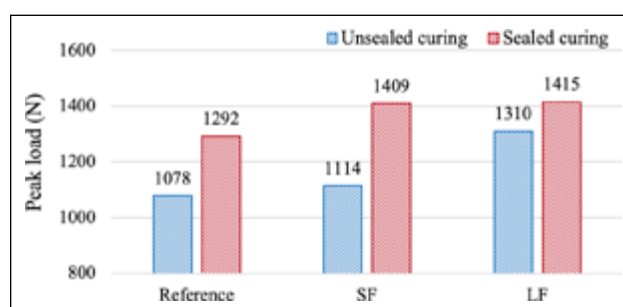
Figure 9. Average peak loads in the fracture energy test.
