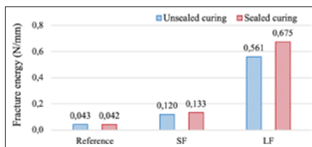
Figure 10. Average fracture energy values in the fracture energy test.
