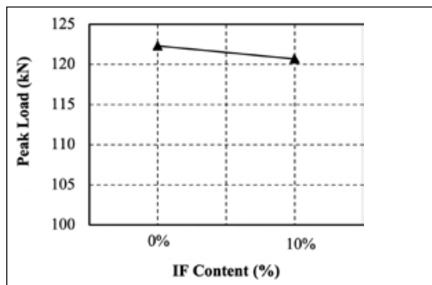
Figure 10. Peak load of beams with IF.
