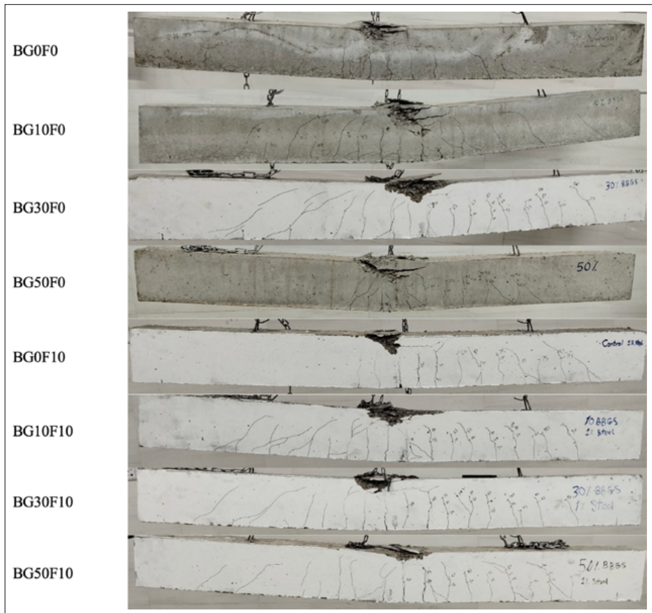
Figure 7. HSRC beams after testing.
