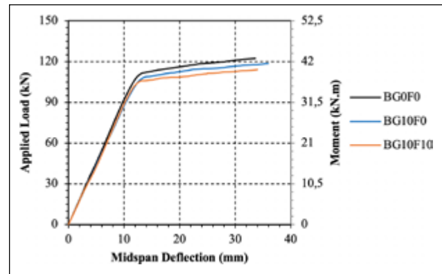
Figure 14. Load-deflection and moment-deflection curves of beams with 10% of GGBS.
