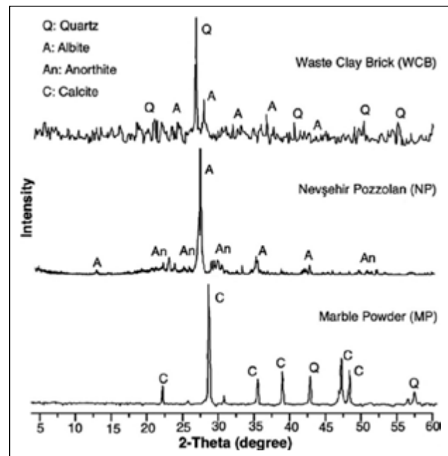
Figure 1. Mineralogical composition of the raw materials (WCB, NP, and MP) by X-ray diffraction (XRD) analysis.
