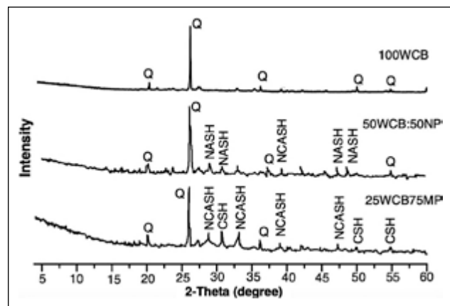
Figure 7. XRD results of one-part alkali-activated mortars.
