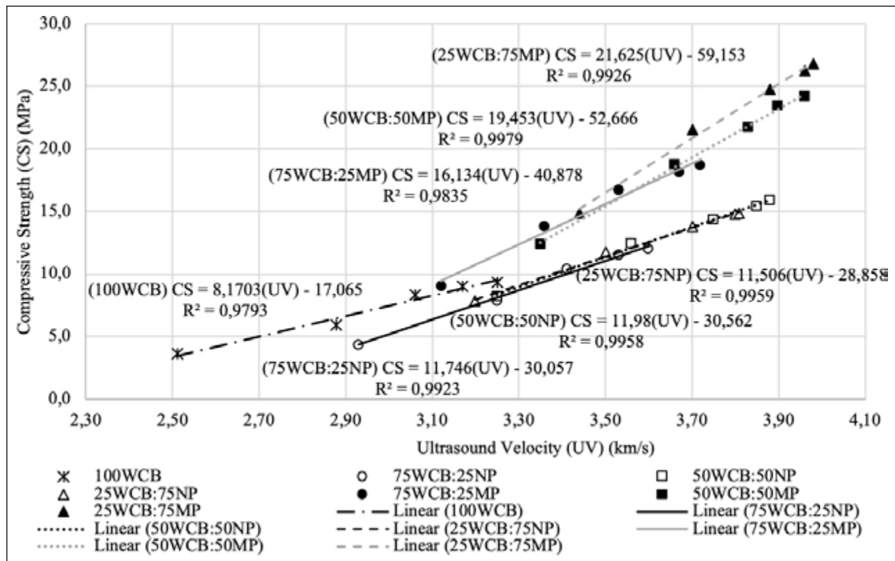
Figure 6. CS of WCB-based one-part alkali-activated mortars as a function of UV.
