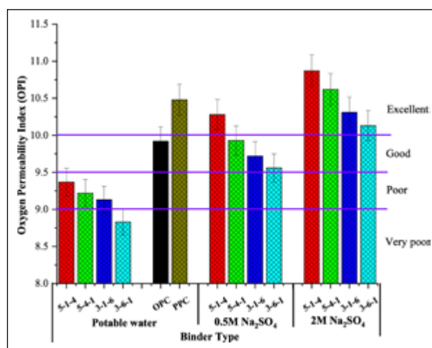
Figure 10. Oxygen permeability index (OPI) results for 0.5 w/c binder mortars cured for 28 days.
