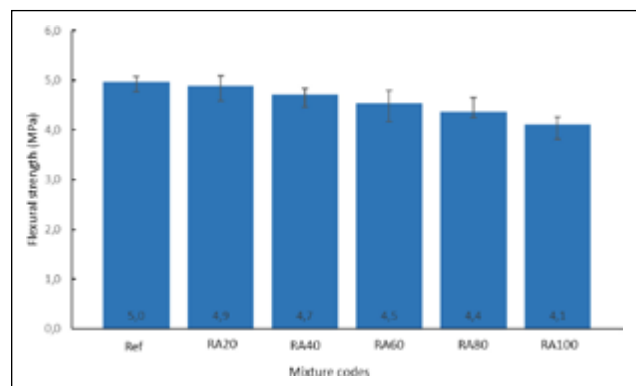
Figure 4. 28-day flexural strength test results.
