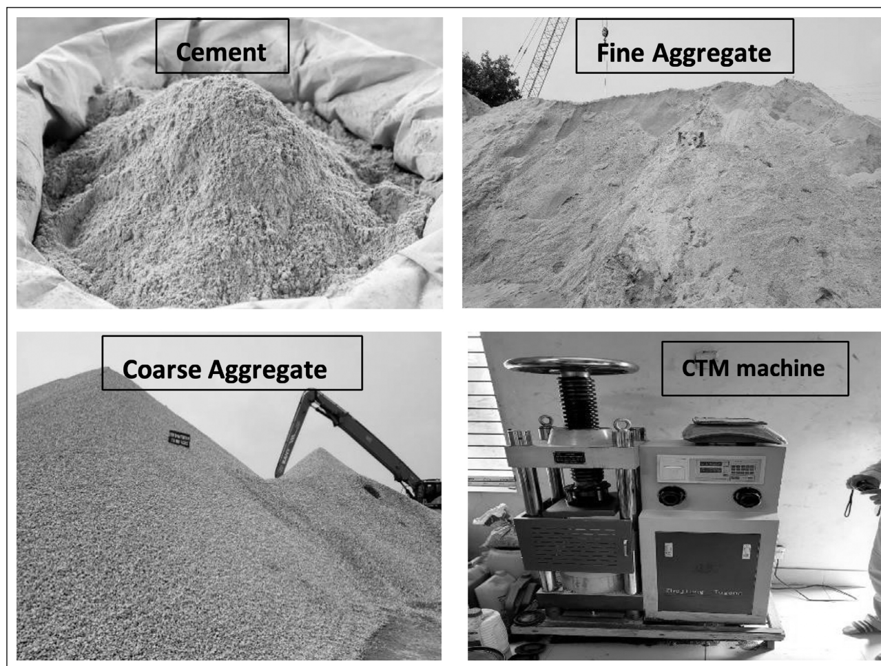
Figure 3. Material and apparatus used for testing.
