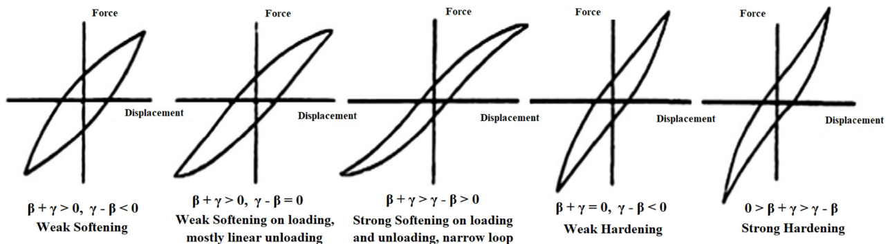
Fig. 6. Possible hysteresis shapes according Bouk-Wen model.
