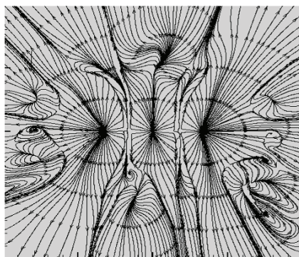
(a) H/D = 1 , Re = 3521.69 Numerical
