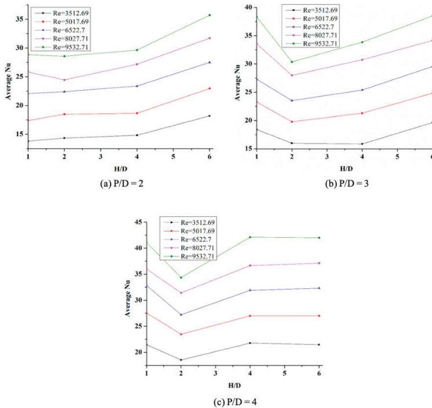
Figure 7. Variation of average Nusselt number.
