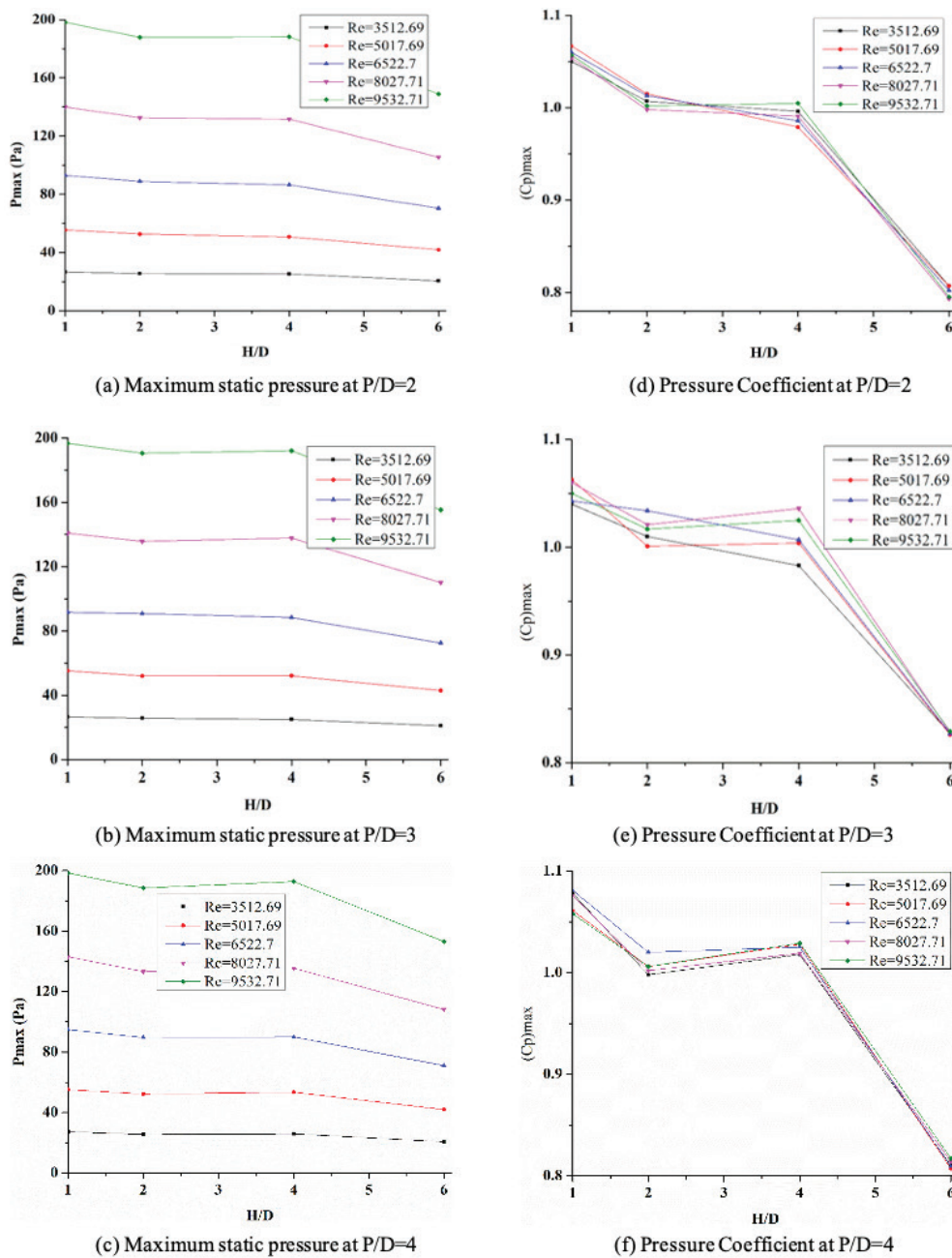
Figure 5. Variation of P_{max} and (C_p)_{max} .
