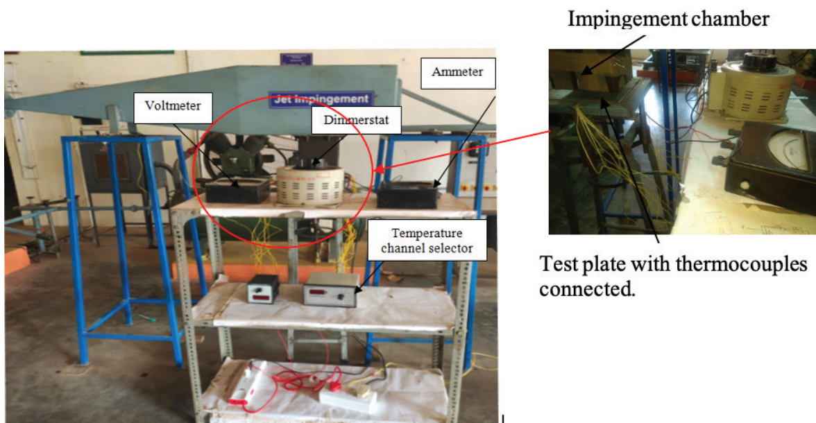
Figure 1. (b) Actual experimental setup.
