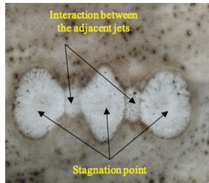
(b) H/D = 1 , Re = 3521.69 Experiment
