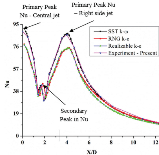
Figure 2. (c) Comparison of turbulence models and validation.
