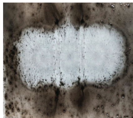
(h) H/D = 2 , Re = 9532.69 Experiment
