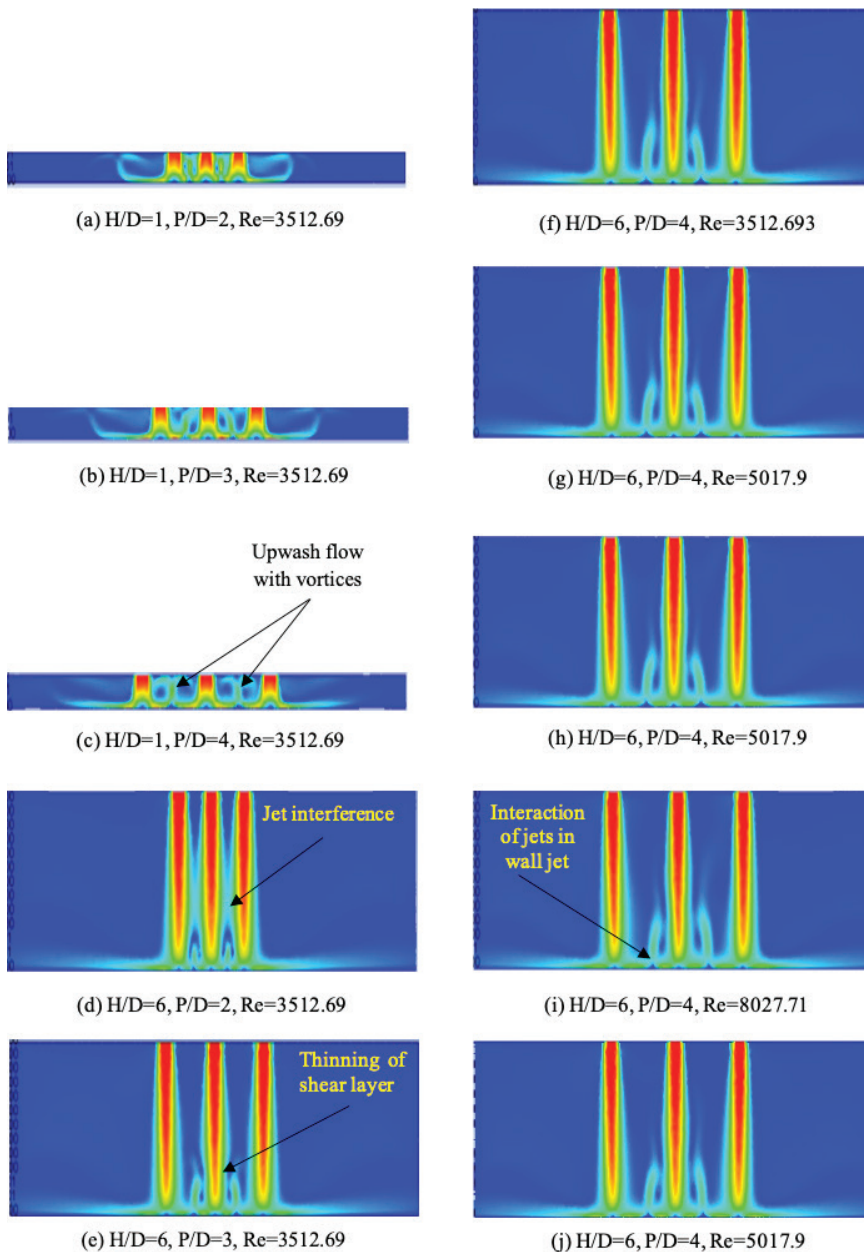
Figure 3. Velocity distributions in the vertical plane passing through the section line X-X.
