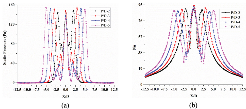
Figure 10. Comparison of static pressure and Nu for H/D=6 , P/D=2, 3, 4 , and 5 at Re=9532.71 .
