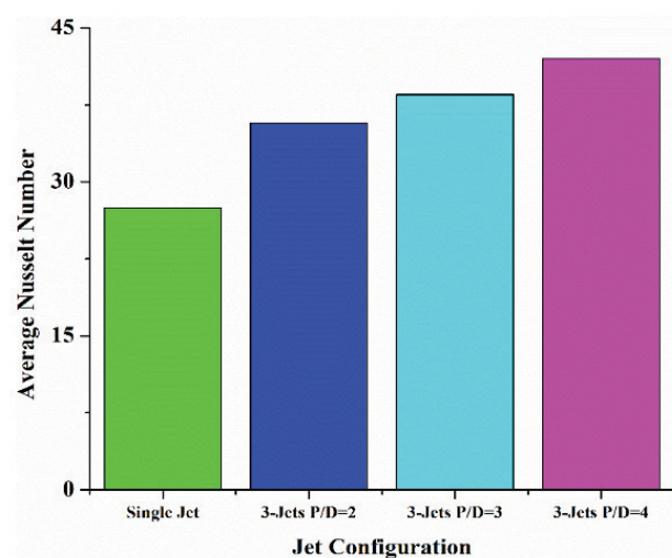
Figure 8. (b) Comparison of average Nusselt number.
