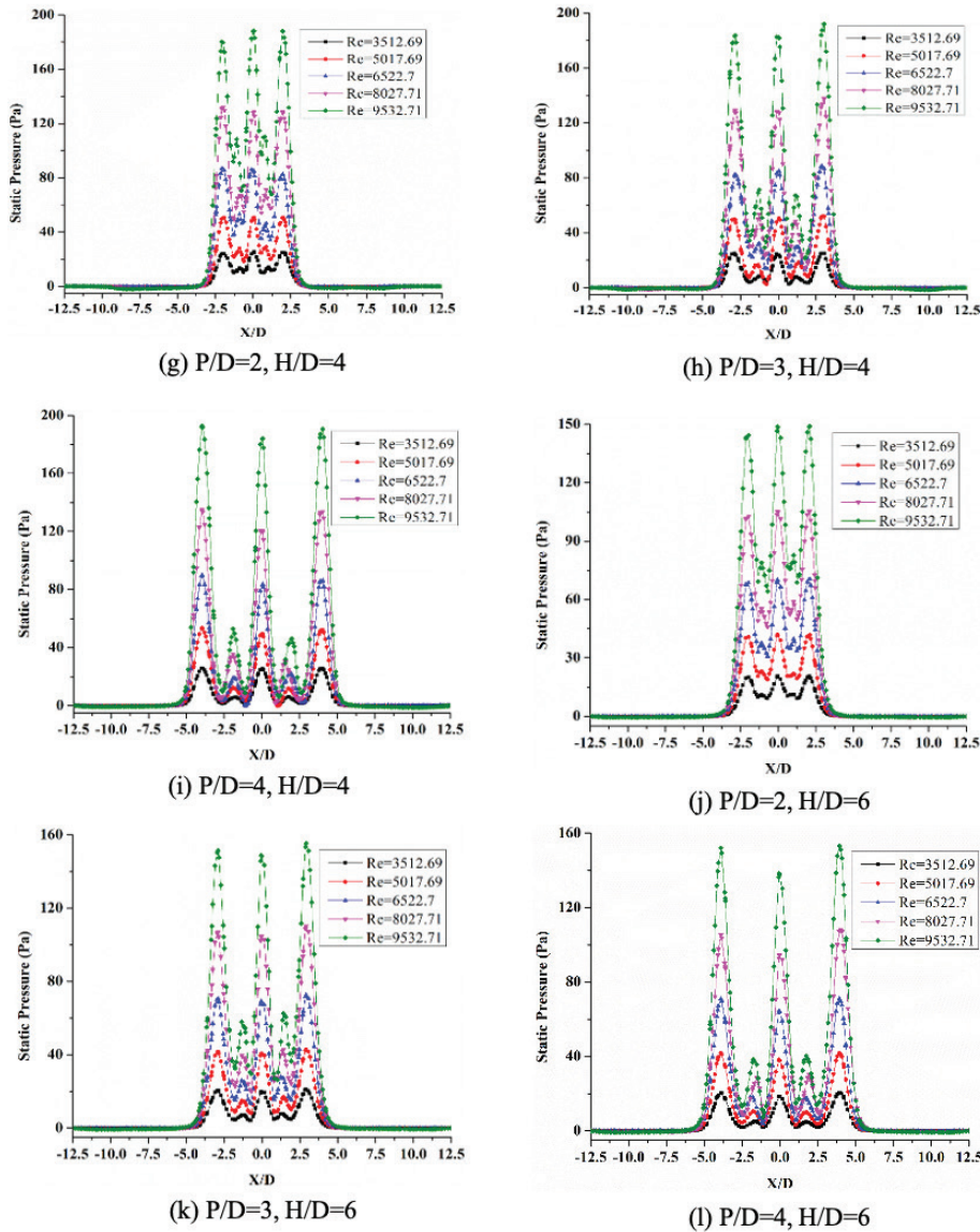
Figure 4. Static Pressure distribution along the section x-x on the target plate.
