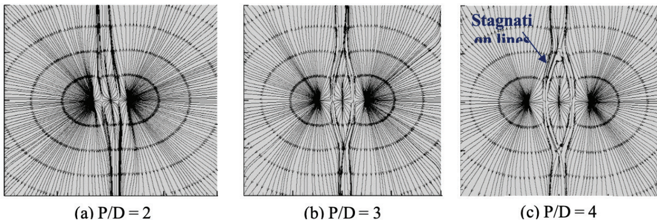
Figure 11. Comparison of flow structures at H/D = 6 , Re = 9532.71 - Numerical analysis.
