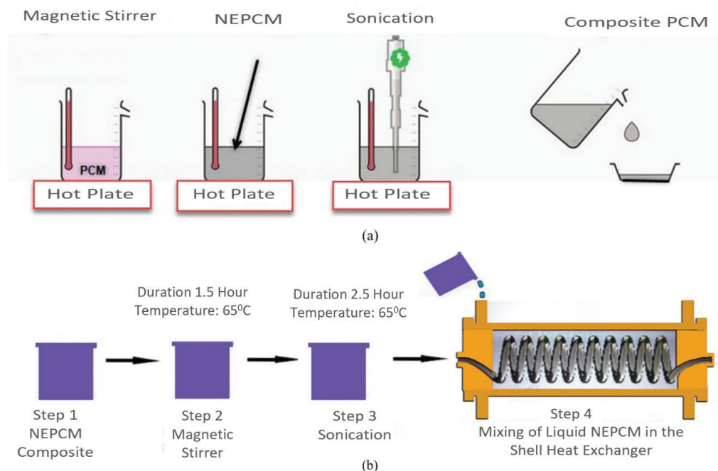
Figure 1. Diagram for preparing samples of NEPCM.
