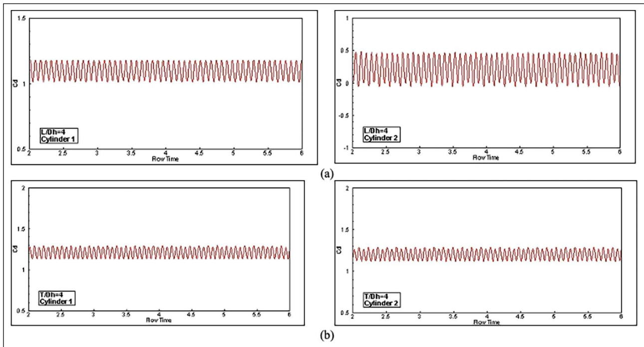
Figure 7. Variation of drag coefficients with flow time for (a) tandem and (b) side-by-side cylinders for L/H=4.0 .
