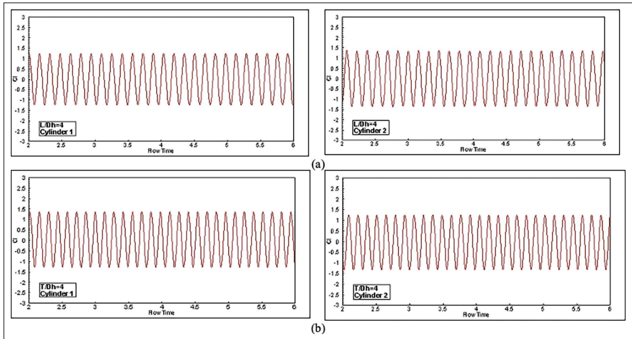
Figure 9. Variation of lift coefficients with flow time for (a) tandem and (b) side-by-side.
