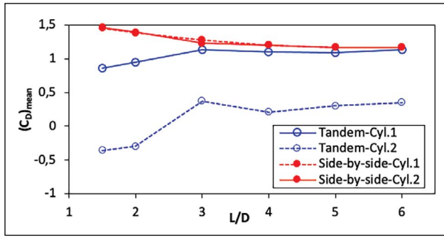
Figure 8. Variation in the mean drag coefficients with gaps between tandem and side-by-side cylinders.
