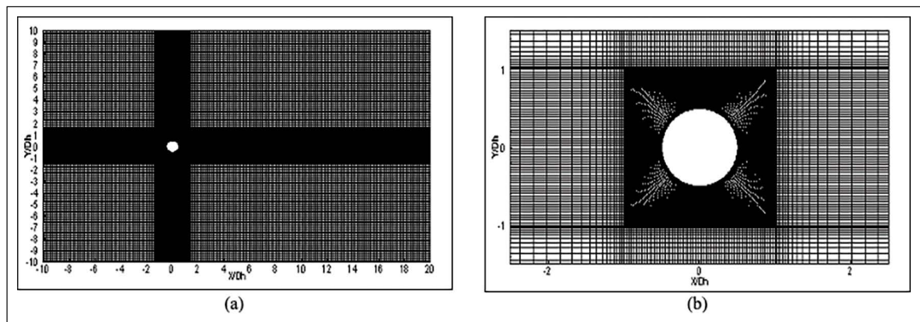
Figure 2. Mesh structure generated in the (a) domain and (b) around each cylinder.
