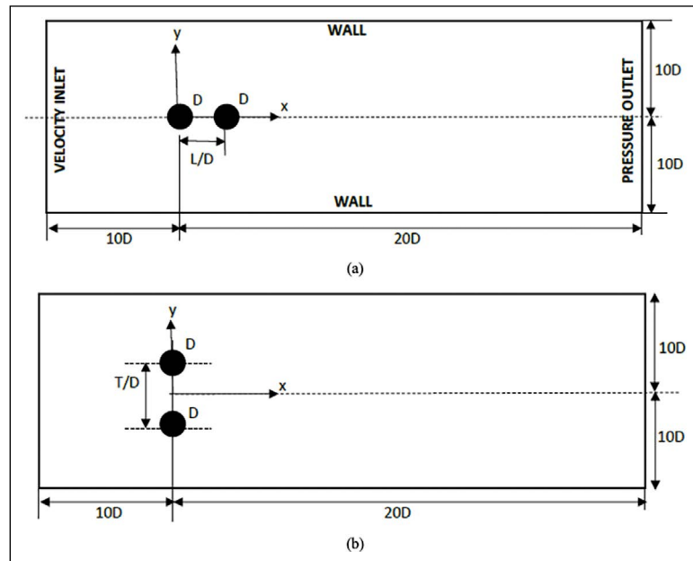
Figure 1. Computational domain for (a) tandem cylinders and (b) side-by-side cylinders (not to scale).
