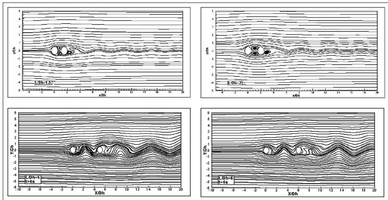
Figure 3. Variation of flow patterns with increasing distance between tandem cylinders.
