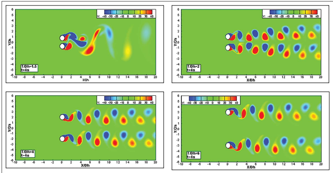
Figure 6. Variation of vorticity with increasing distance between side-by-side cylinders.
