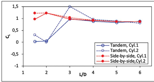
Figure 10. Variation in the mean lift coefficients with gaps between tandem and side-by-side cylinders.
