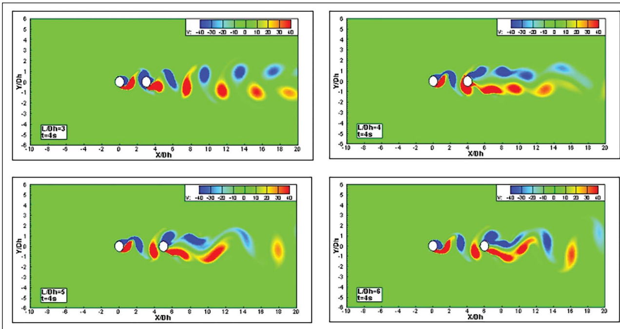
Figure 5. Variation of vorticity with increasing distance between tandem cylinders.
