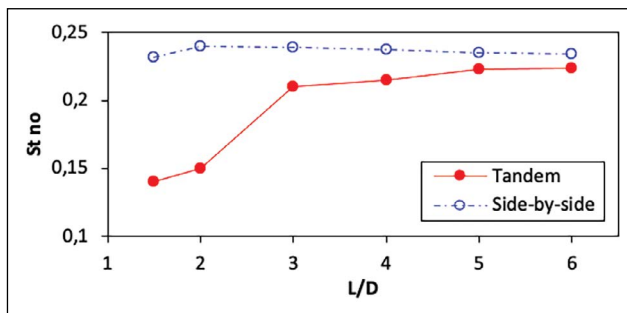
Figure 11. Variation in the Strouhal (St) number with gaps between tandem and side-by-side cylinders.
