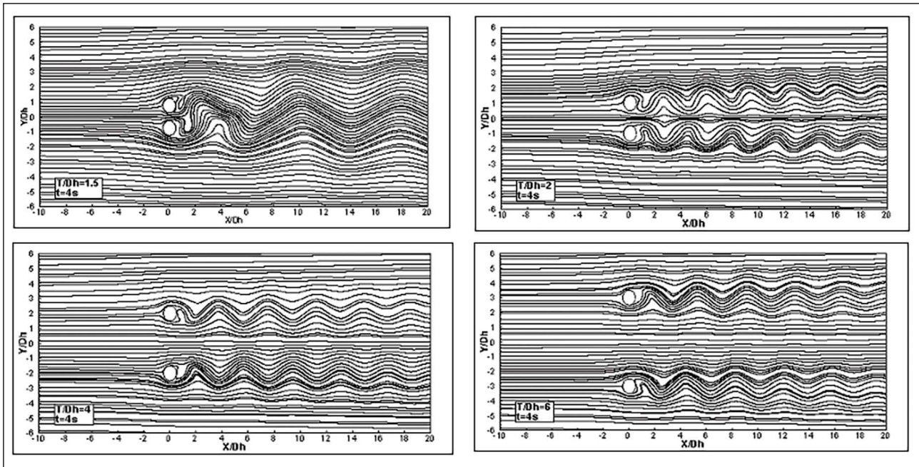
Figure 4. Variation of flow patterns with increasing distance between side-by-side cylinders.
