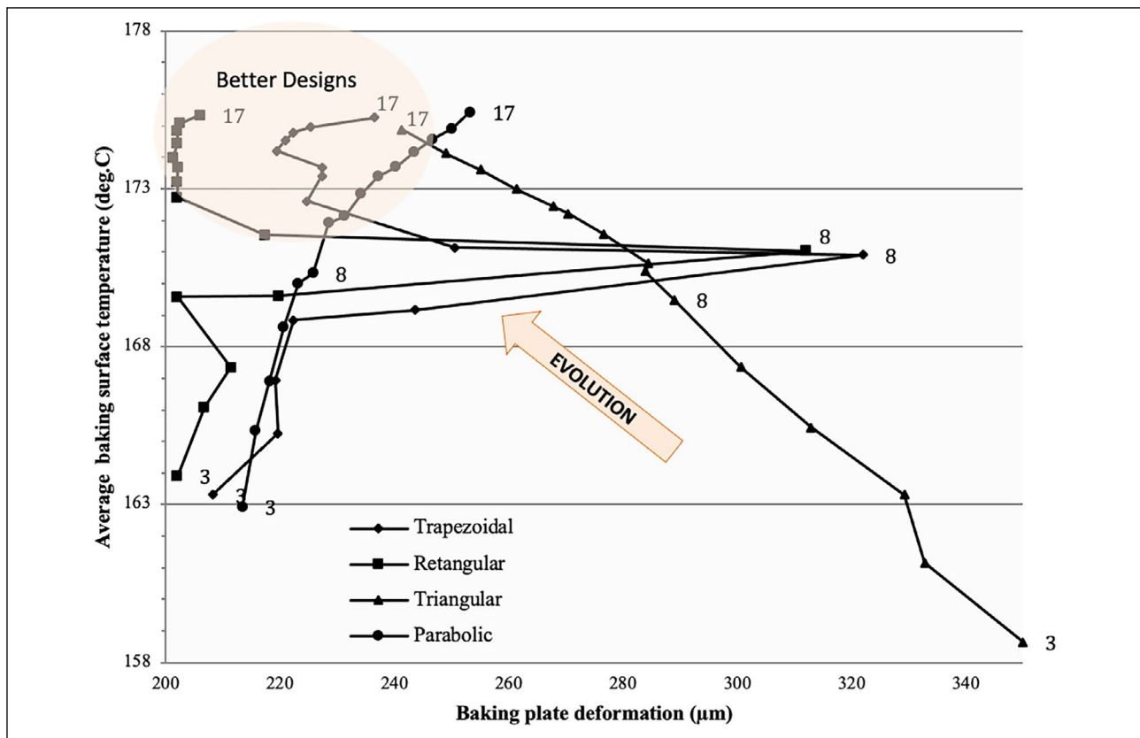
Figure 13. Overview of the trade-off between the maximum baking plate deformation versus the average baking surface temperature for all configurations tested.
