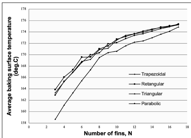
Figure 10. Average baking surface temperature of the plate finned with variable number of trapezoidal, triangular parabolic and rectangular fins.
