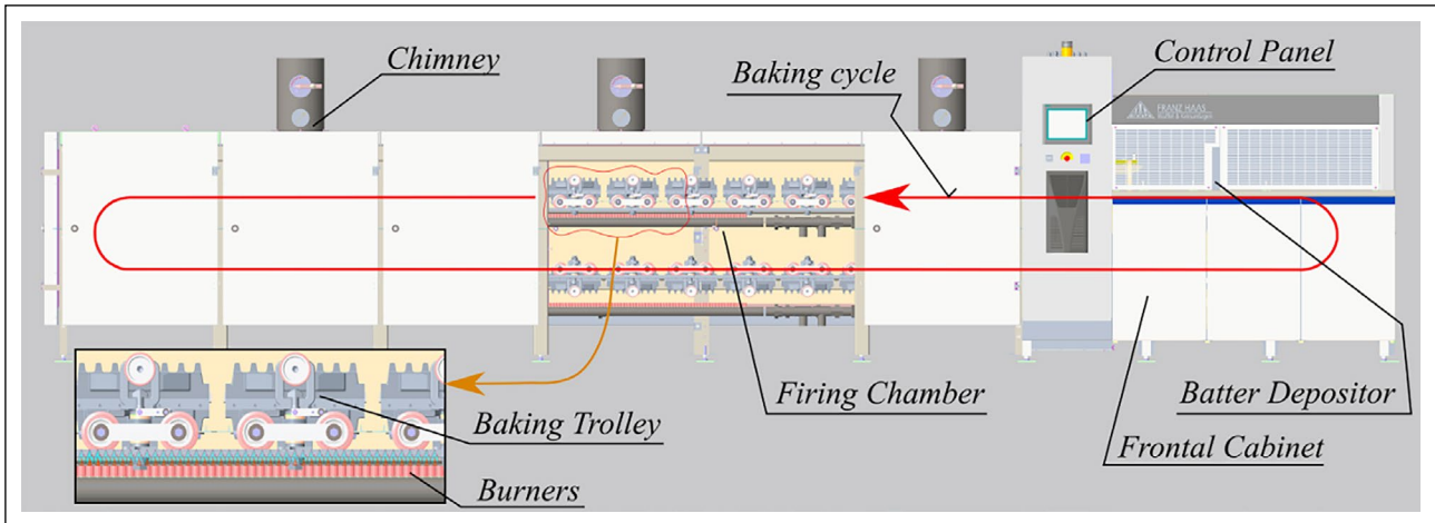
Figure 1. Schematics of an industrial flat wafer gas oven showing the baking sheets boarded on trolleys that travel along rails as a train. Burners are lined transversally to the rails. The travel cycle ends in the loading and unloading cabinet (rightmost side).
