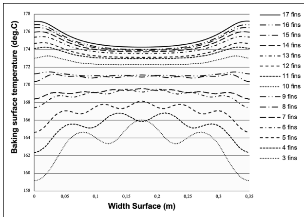
Figure 6. Temperature profile along the width of the baking surface of the plate for trapezoidal shape for different numbers of fins, N .
