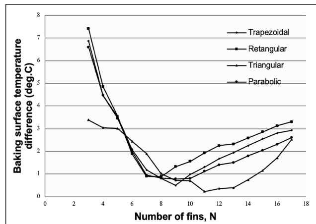
Figure 11. Difference between maximum and minimum temperature at baking surface of the plate finned with variable number of trapezoidal, triangular parabolic and rectangular fins.
