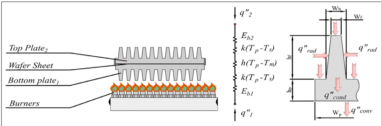
Figure 2. Schematic drawing of a baking plate with the line of burners, the heat transfer circuit analogy and a one-rectangular fin slice of the baking plate and the main dimensions.
