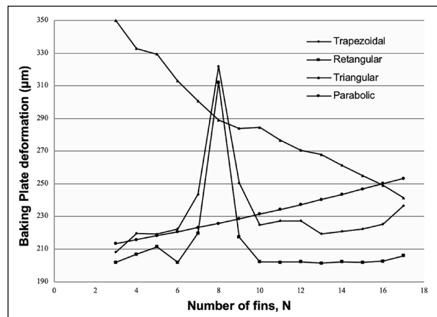
Figure 12. Maximum deformation \delta of the baking plate due baking pressure caused by the steam generation from the baking dough.
