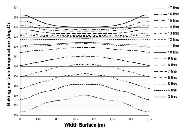
Figure 7. Temperature profile along the width of the baking surface of the plate for triangular shape for different numbers of fins, N .
