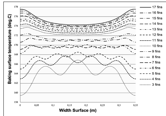
Figure 8. Temperature profile along the width of the baking surface of the plate for rectangular shape for different numbers of fins, N .
