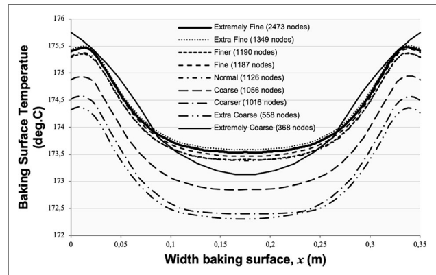
Figure 5. Temperature profile along the width of the baking surface of the plate with 13 trapezoidal fins with different mesh sizes.
