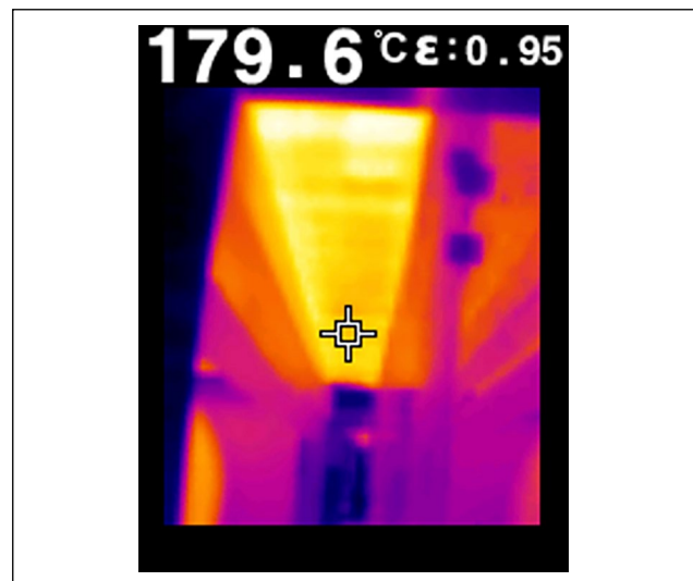
Figure 3. Thermographic images of the top baking plate during operation shows 179.6°C, the emissivity adjusted to measure with 0.95.
