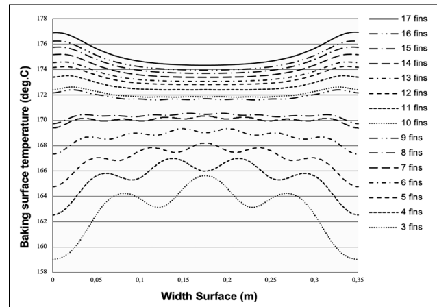
Figure 9. Temperature profile along the width of the baking surface of the plate for parabolic shape for different numbers of fins, N .
