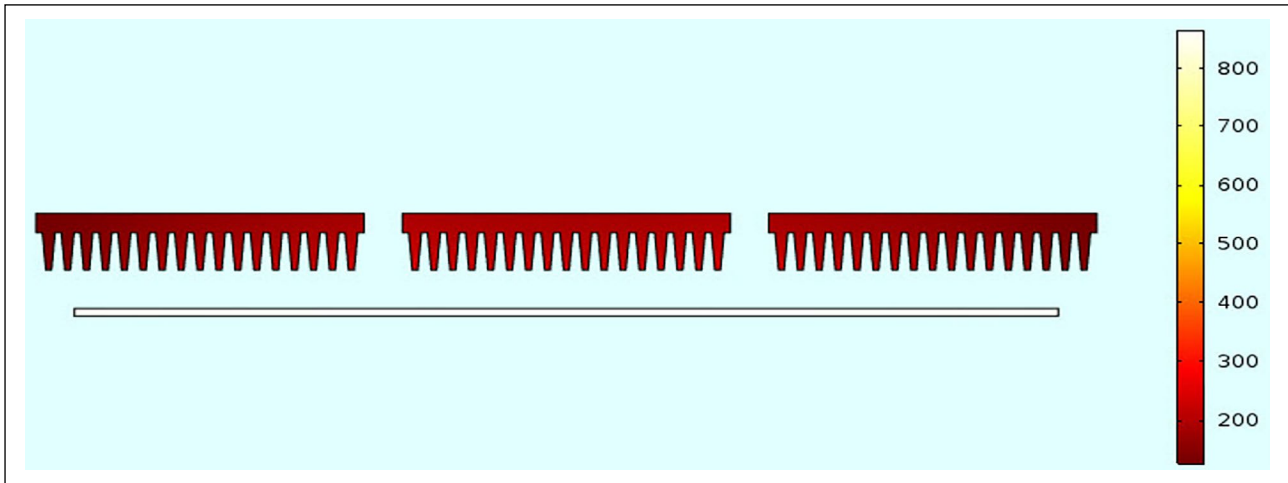
Figure 4. Illustration of the temperature field of the middle plate (the observed part of the simulation) with 17 trapezoidal fins and the flat radiant “flame”.
