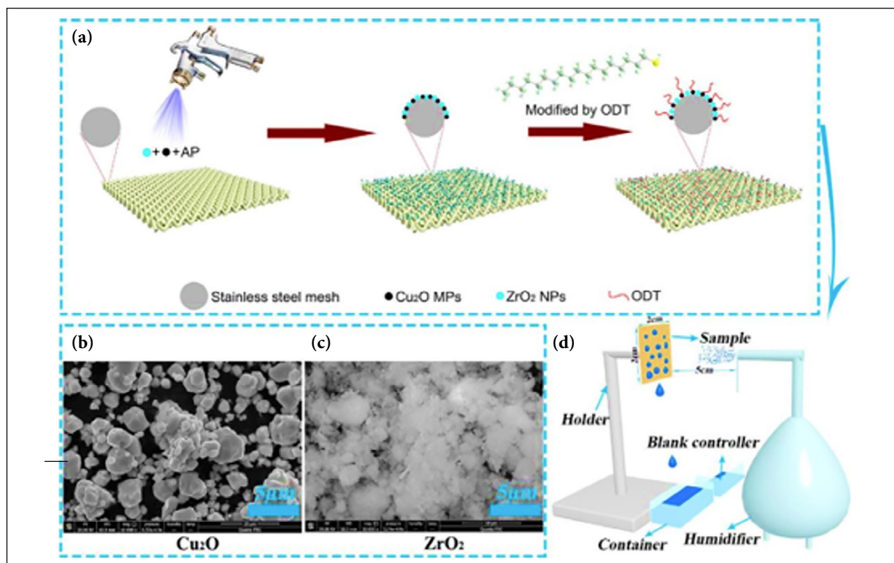
Figure 36. (a) Schematic demonstration of the fabrication process of hybrid super-hydrophilic super-hydrophobic surface (b, c) Scanning Electron Microscopy images of \text{Cu}_2\text{O} and \text{ZrO}_2 . (d) The setup apparatus to catch the fog during the fog harvesting experiments (Feng et al, 2020).
