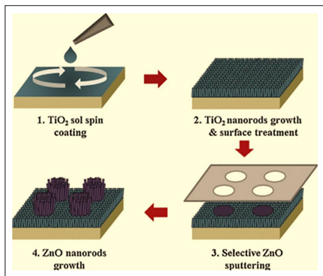
Figure 30. Schematic illustration of the fabrication of a superhydrophilic ZnO/ superhydrophobic \text{TiO}_2 surface (Choo et al, 2015).
