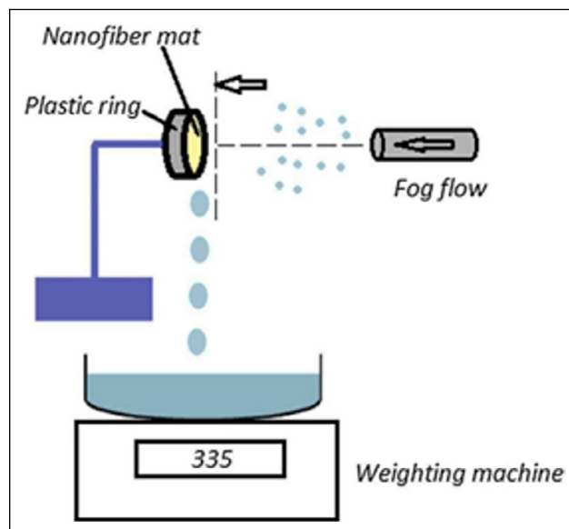
Figure 29. The schematic of the used system (Almasian et al, 2018).
