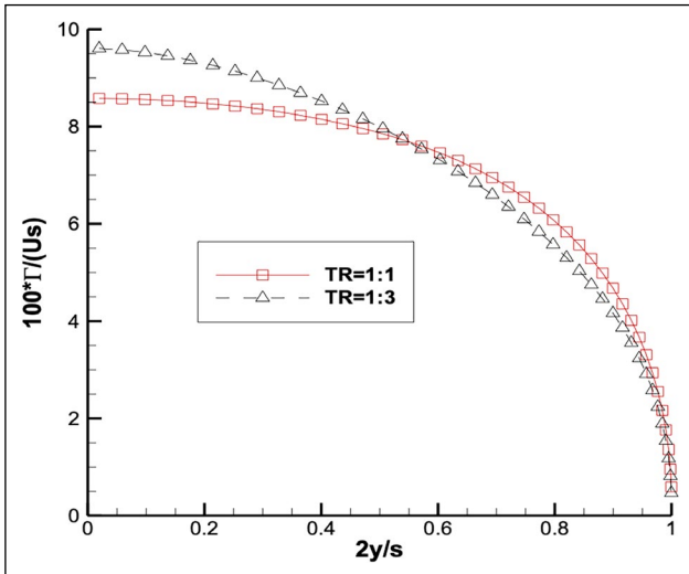
Figure 6. Non-dimensional circulation distribution of rectangular hydrofoil and tapered hydrofoil with no cavitation and no free surface effects. Only half of the distributions are shown due to symmetry.
