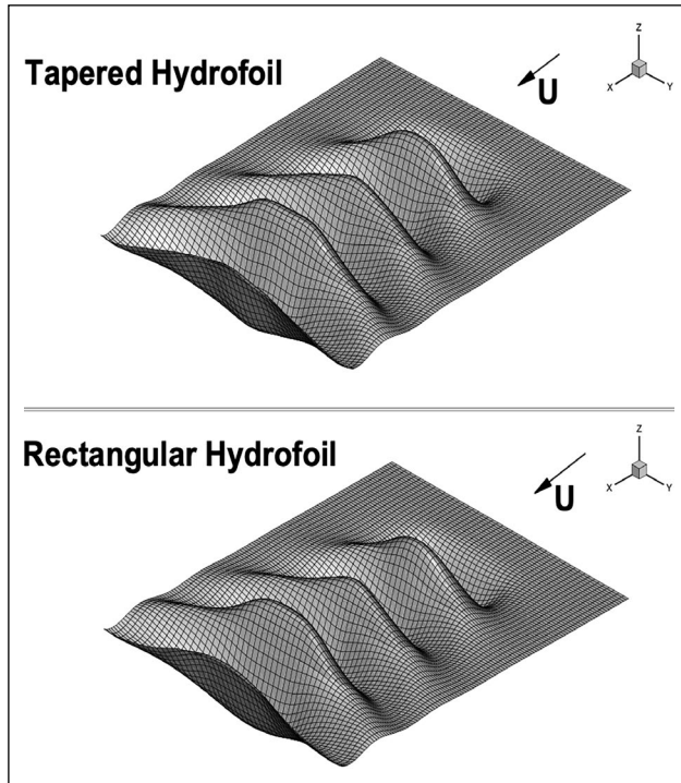
Figure 11. Wave deformation on free surface for both hydrofoils; \alpha=5^\circ , \sigma=0.7 , h/c_m=1.0 , Fr_c=0.8 .
