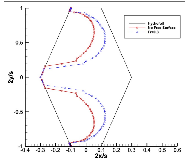
Figure 10. Cavity planforms for tapered hydrofoil, \alpha=5^\circ , \sigma=0.7 , h/c_m=1.0 .
