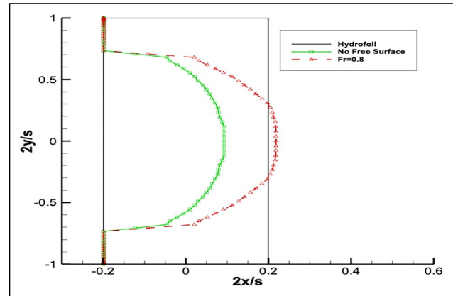
Figure 9. Cavity planforms for rectangular hydrofoil, \alpha=5^\circ , \sigma=0.7 , h/c_m=1.0 .
