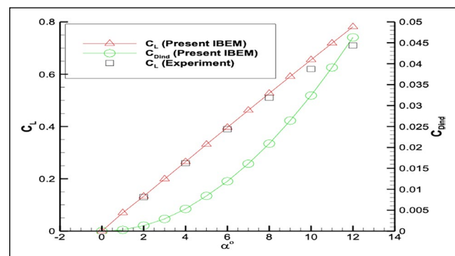
Figure 3. Comparison of lift coefficients with experiments.
