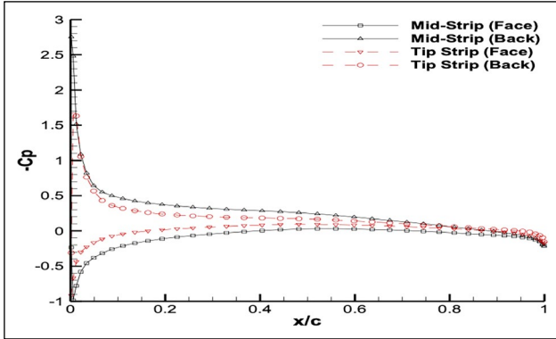
Figure 4. The non-dimensional pressure distribution on mid-section and tip section.
