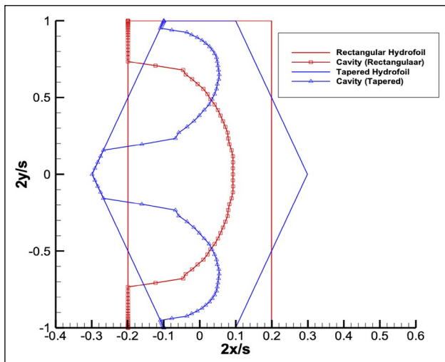
Figure 8. Cavity planforms for rectangular and tapered hydrofoils in unbounded flow domain, \alpha=5^\circ , \sigma=0.7 .
