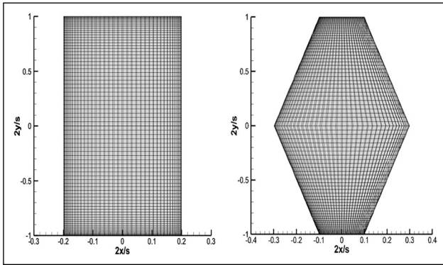
Figure 5. The rectangular (left) and tapered (right) hydrofoils with panels used in the calculations.
