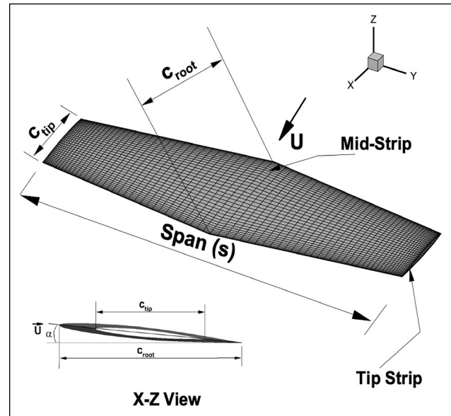
Figure 2. Parameters and panels on the tapered hydrofoil used for validation.
