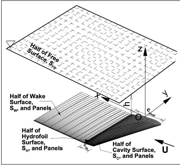
Figure 1. Coordinate system for the 3-D cavitating hydrofoil problem. Only half of the hydrofoil, its wake, and free surface are shown due to the property of symmetry.
