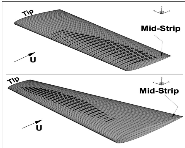
Figure 7. Cavity shapes for rectangular (up) and tapered (down) hydrofoils in unbounded flow domain. Only half of the distributions have shown due to symmetry, \alpha=5^\circ , \sigma=0.7 .
