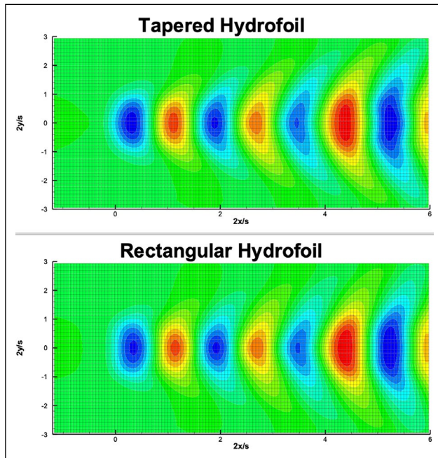
Figure 12. Kelvin wave contours on free surface for both hydrofoils; \alpha=5^\circ , \sigma=0.7 , h/c_m=1.0 , Fr_c=0.8 .
