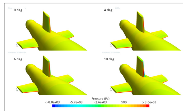
Figure 16. Pressure Distribution on Aft Body of Submarine.
