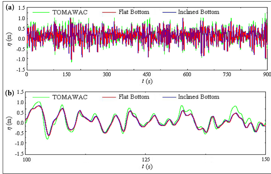
Figure 4. Qualitative comparison of the results obtained in the first analysis considering realistic irregular waves at the probe located at x=0 m: (a) 0 \leq t \leq 900 s; (b) 100 \leq t \leq 150 s.
