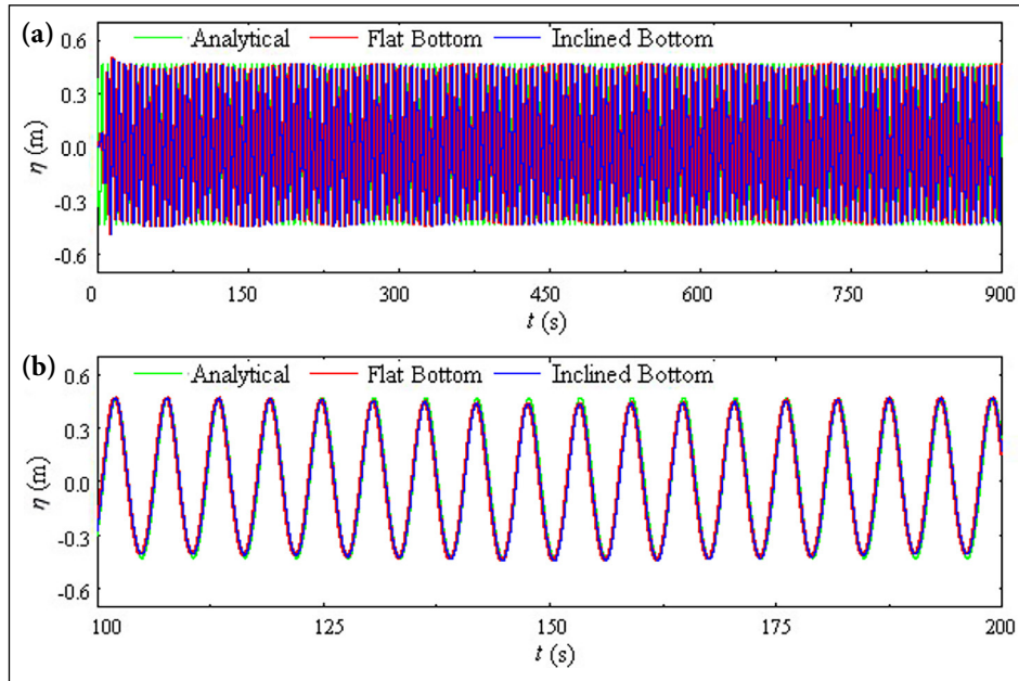
Figure 7. Qualitative comparison of the results obtained in the first analysis considering representative regular waves at the probe located at x=41.82 m: (a) 0 \leq t \leq 900 s; (b) 100 \leq t \leq 200 s.
