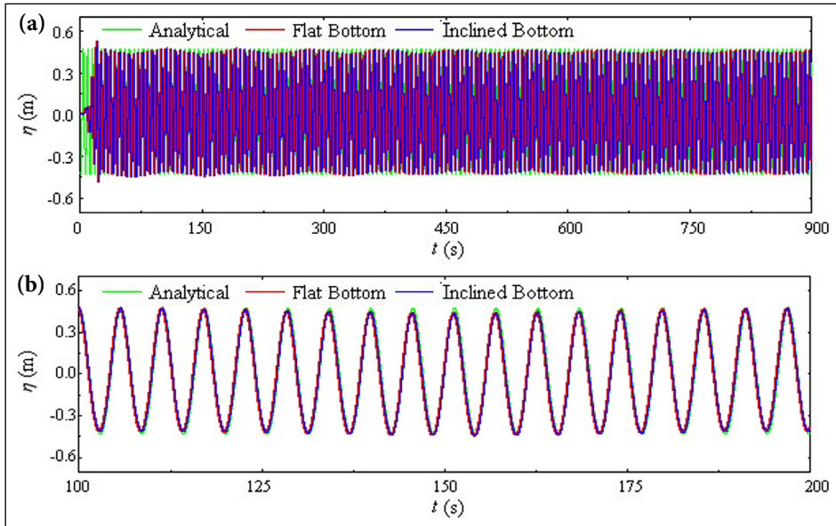
Figure 8. Qualitative comparison of the results obtained from the first analysis considering representative regular waves at the probe located at x=71.09 m: (a) 0 \leq t \leq 900 s; (b) 100 \leq t \leq 200 s.
